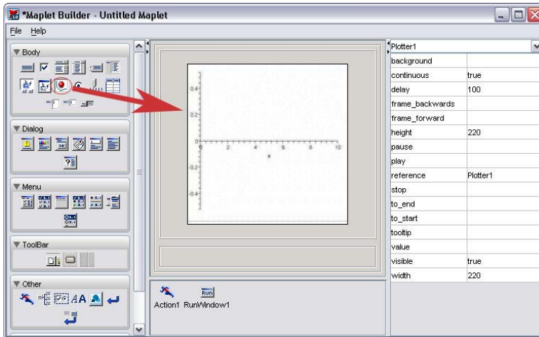
Figure 9.6: Add a Plot to Row 1
