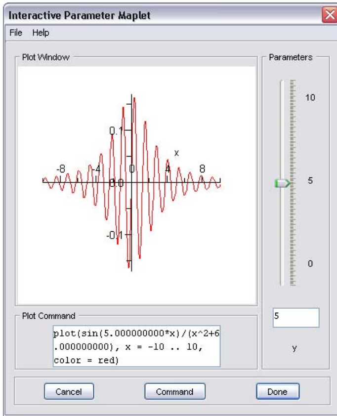
Figure 5.1: Interactive Parameter Window
