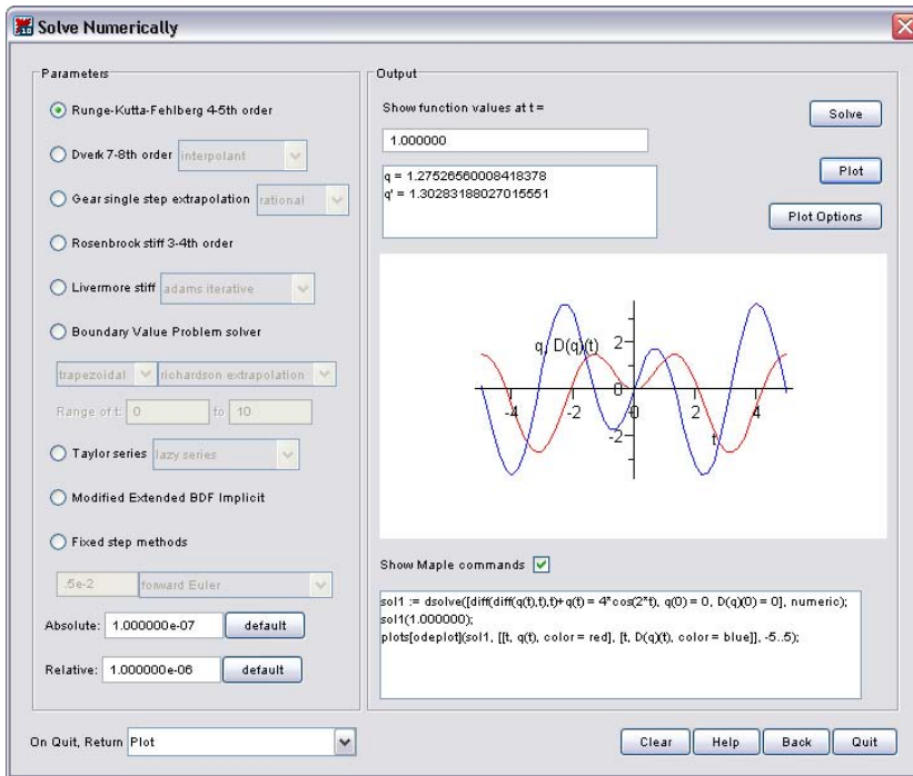
Figure 3.4: ODE Analyzer Assistant: Solve Numerically Dialog
