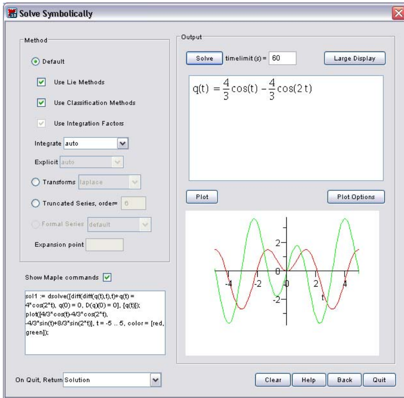
Figure 3.5: ODE Analyzer Assistant: Solve Symbolically Dialog
