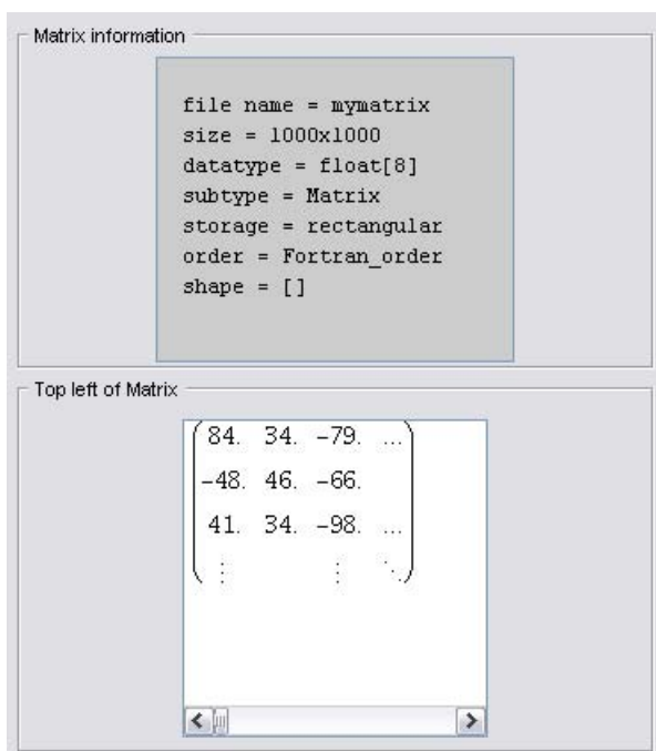
Figure 10.1: Import Data Assistant (Detail)
