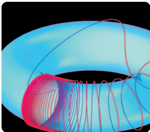
Gauss Map Graphed on a Torus
