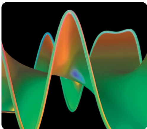
Dirichlet Problem for a Circle
