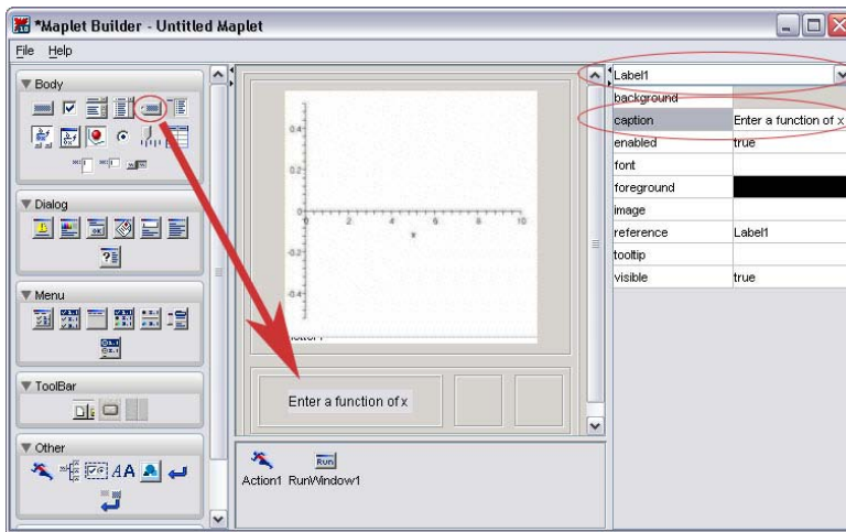
Figure 9.8: Add a Label to Row 2
