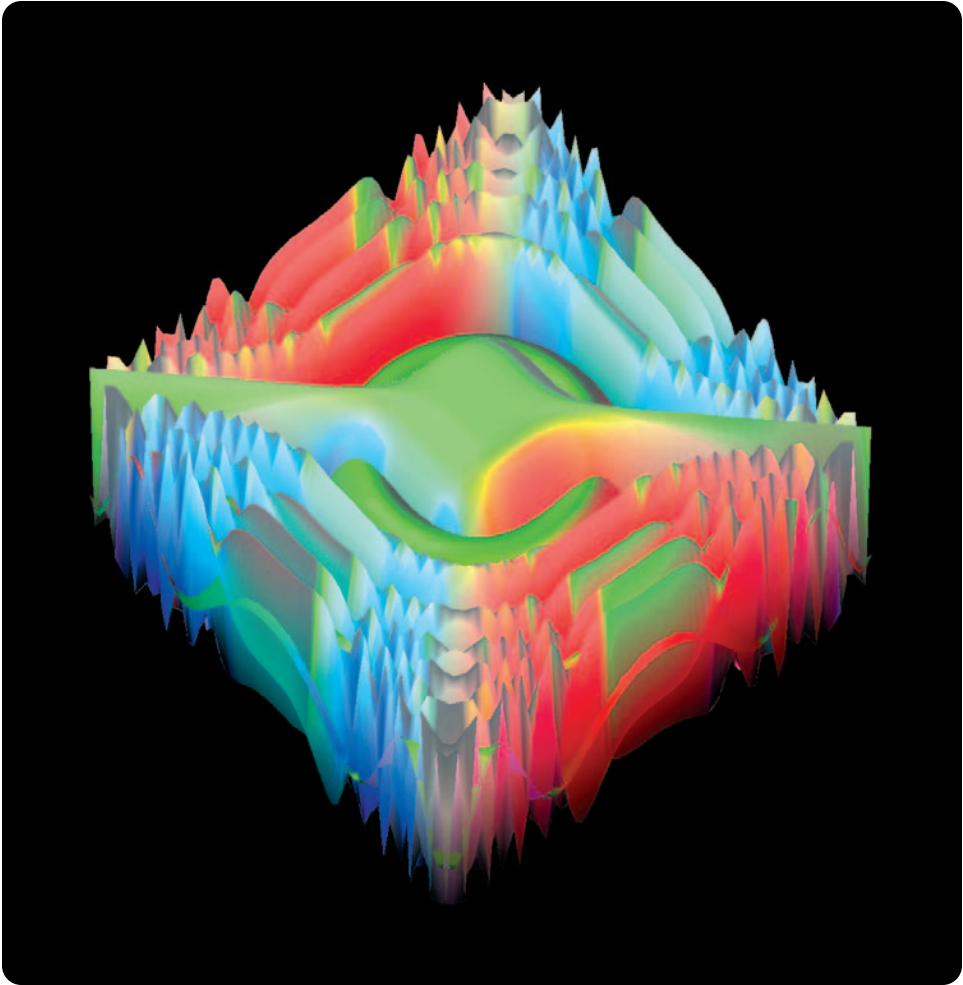
Function of Two Variables in Cartesian Coordinates
