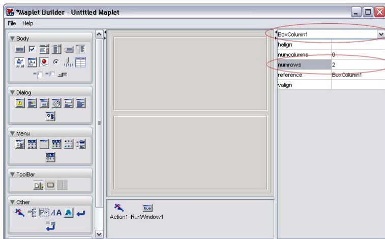
Figure 9.5: Define the Number of Rows in the Maplet
