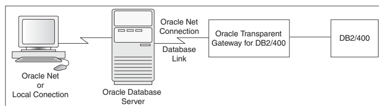
Figure 1–1 Architecture of the Oracle Transparent Gateway for DB2/400
